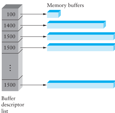
Figure 2.43 Buffer descriptor list.
