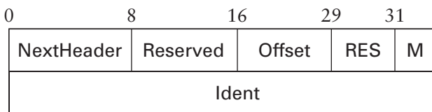
Figure 4.35 IPv6 fragmentation extension header.
