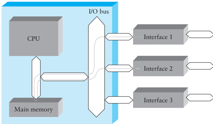
Figure 3.27 A workstation used as a packet switch.
